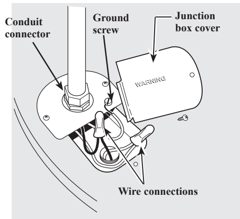
Water heater junction box
